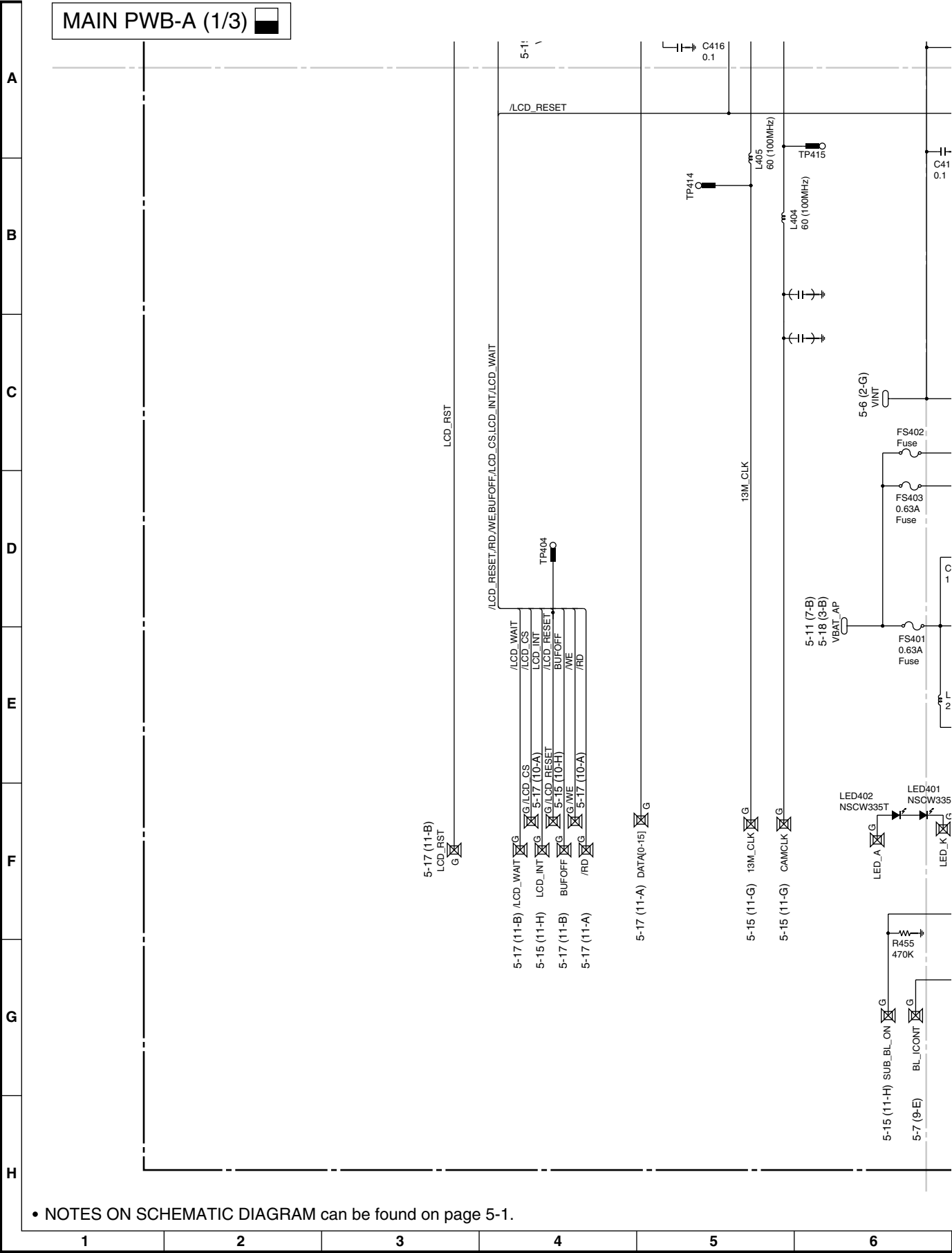
Figure 3 SCHEMATIC DIAGRAM (3/24)
