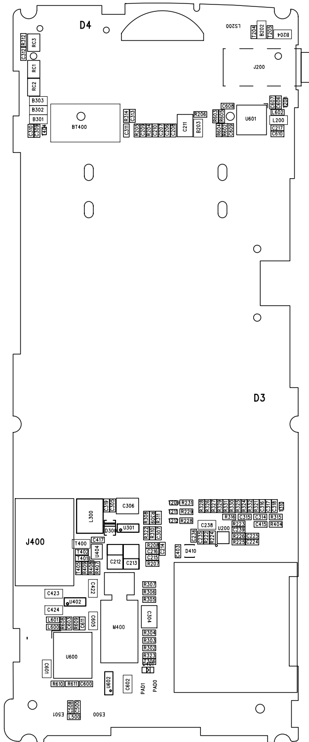
WG803_MAINBOARD_V3.0_ASSEMBLY_BOT_2006/09/08
